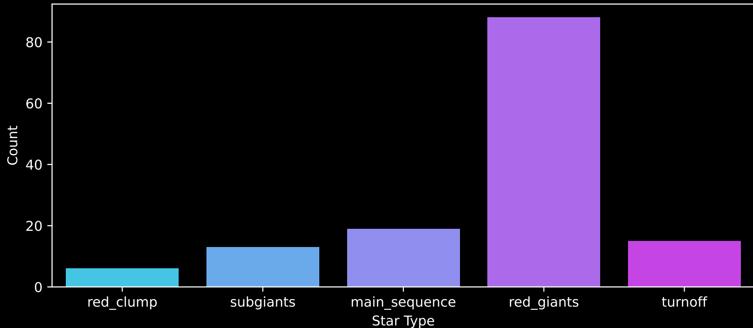
APOGEE DR17 Field: [010+00] Count plot of Star Type
