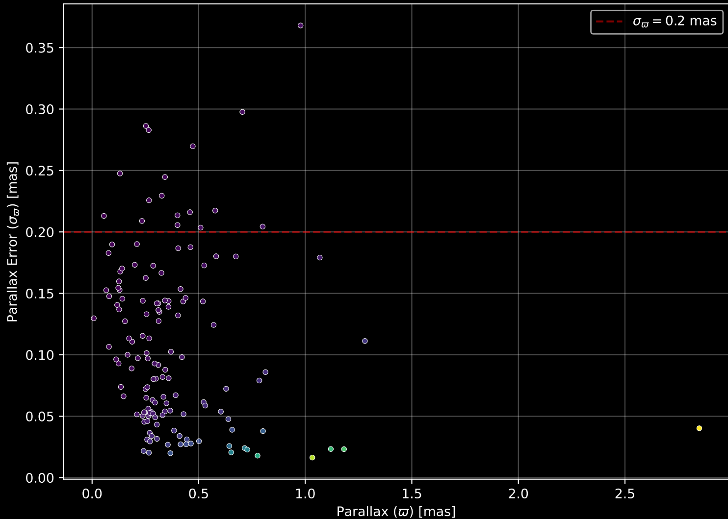
APOGEE DR17 Field: [010+00] Parallax Quality (n= 141)
