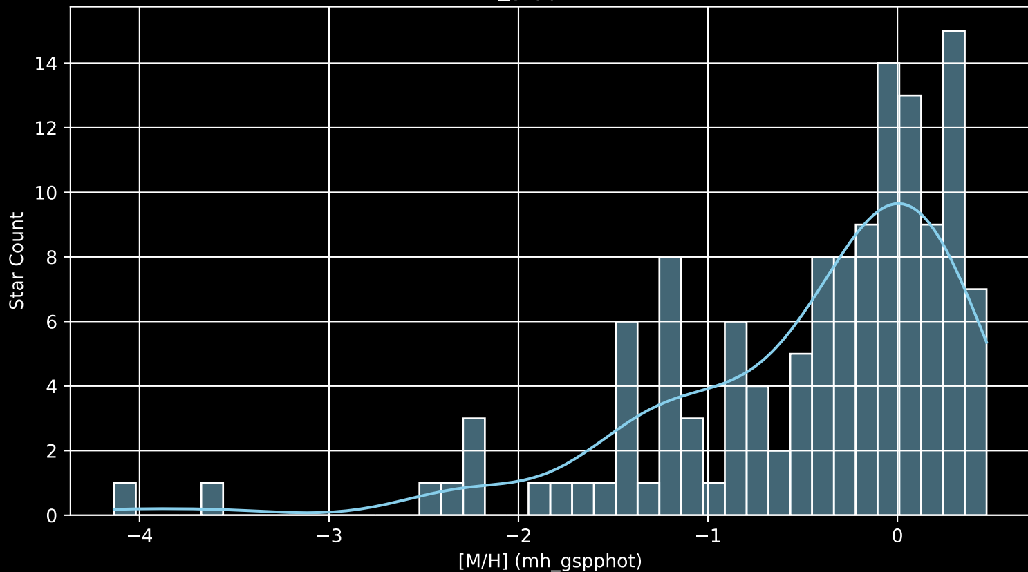
APOGEE DR17 Field: [010+00 [M/H] (mh_gspphot) (n= 130)
