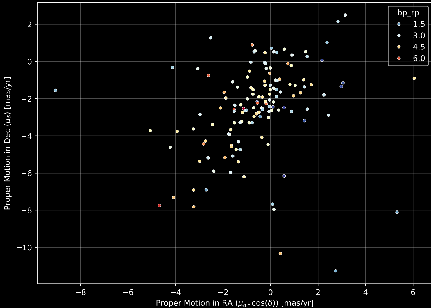
APOGEE DR17 Field: [010+00] Proper Motion Diagram (n= 141)
