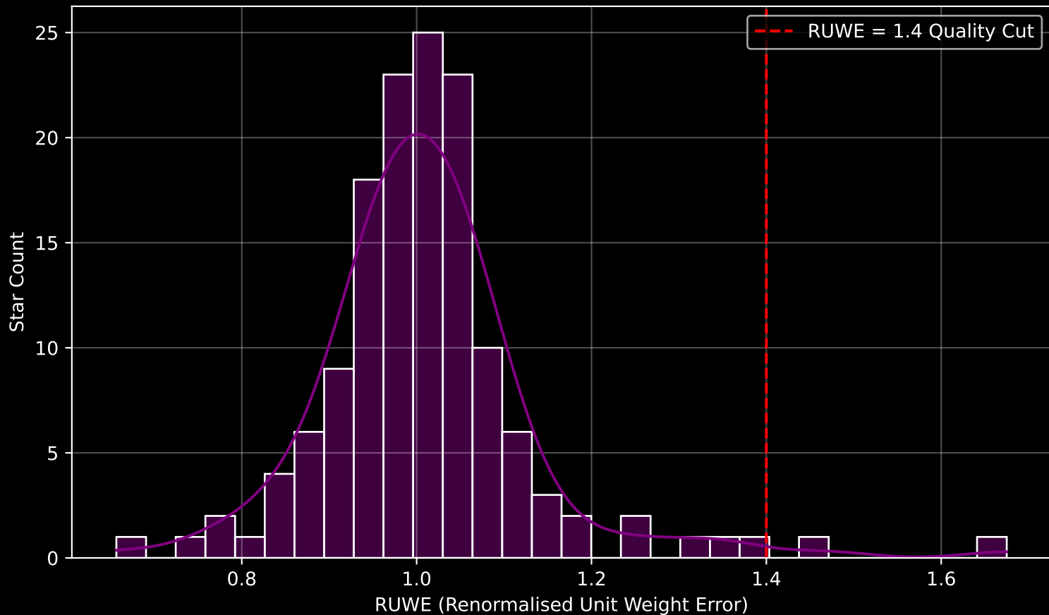
GAPOGEE DR17 Field [010+00] RUWE Distribution (n= 141)
